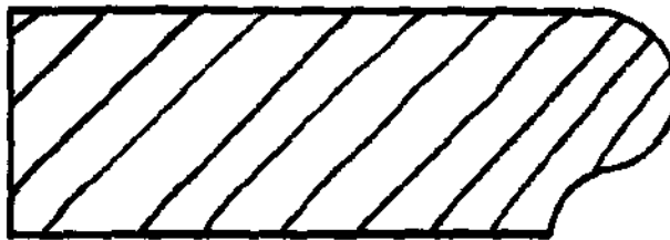
RB 9891-3-1/8 WOODHAVEN WINDOW STOOL 1-1/16" x 3-1/8"
