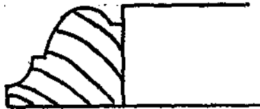
RADCLIFF PANEL MOULD RB 9859 3/4" x 7/8"
