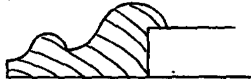
CHATEAU PANEL MOULD RB 9849 3/4" x 1 5/8"
