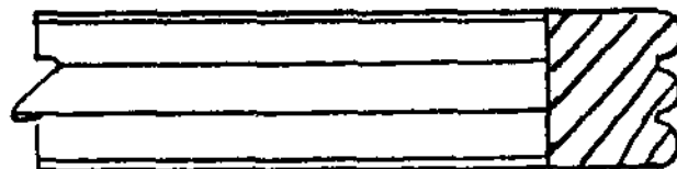
RB 9881-3/4 HANOVER SHELF EDGE 5/8" x 3/4"
