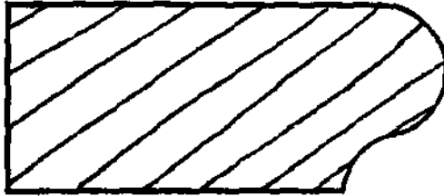
RB 9891-2-1/2 WOODHAVEN WINDOW STOOL 1-1/16" x 2-1/2"
