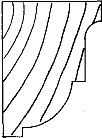
RB 9897 TUSCAN CAPITAL MOULD 1 3 / 4 " x 2 3 / 8 "
