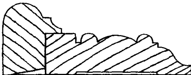
RB 9902 TOWNSEND BACK BAND 1 1/16" x 1 5/16"
