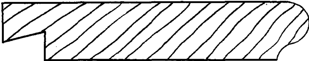
RB 9892-5 1 / 2 " RODENHAVEN WINDOW STOOL 1 1 / 16 " x 5 1 / 2 "
