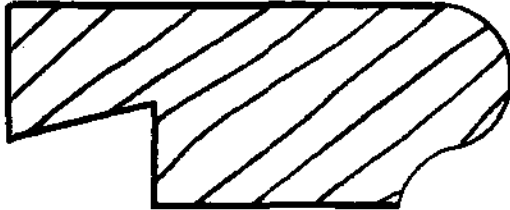
RB 9892-2 5 / 8 " RODENHAVEN WINDOW STOOL 1 1 / 16 " x 2 5 / 8 "
