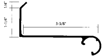
3 3/8" Female Hinge
