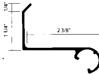
2 3/8" Female Hinge
